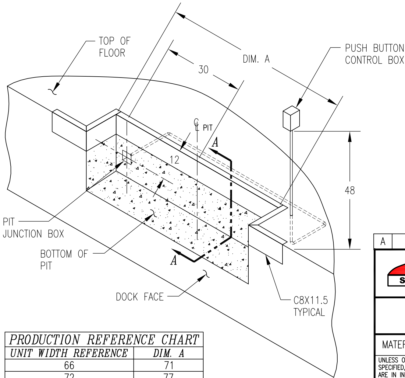
ISOMETRIC VIEW
